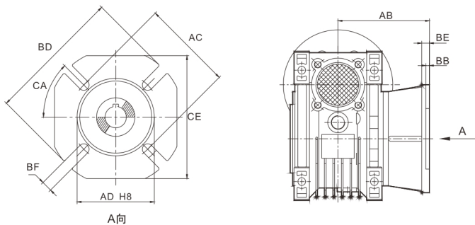
输出法兰安装尺寸 Output Flange Mounting Dimensions
