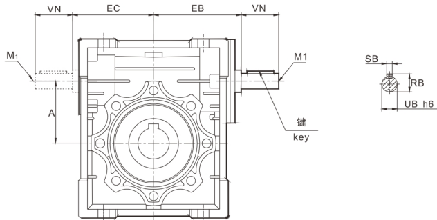
JRST(B)安装尺寸 JRST(B) Mounting Dimensions
